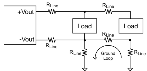
Fig.17 Ground Loops
