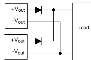
Fig.22 Redundant Operation
