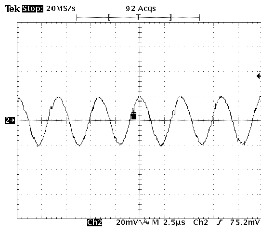
Typical Output Ripple Voltage AV45C-048L-050F20HAN
