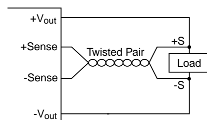
Fig.9 Sense Connections
