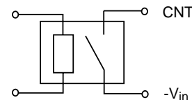
Fig.8 Relay CNT Control
