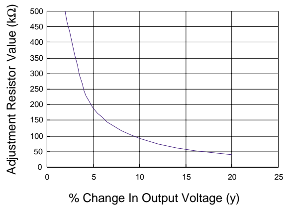
Fig.14 Resistor Selection for Trimming Down Output
