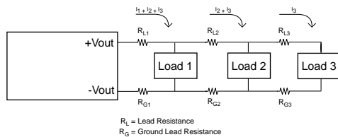
Fig.19 Parallel Power Distribution
