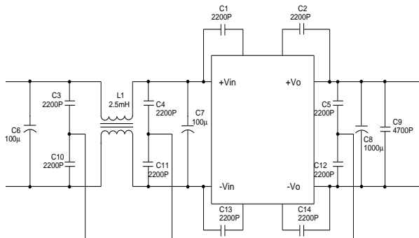
Fig.4 EMI Reduction Input Filter
