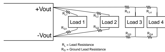
Fig.21 Mixed Power Distribution
